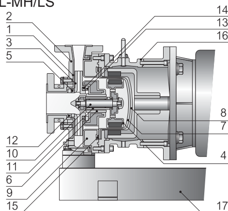
TSL-MH/LS
